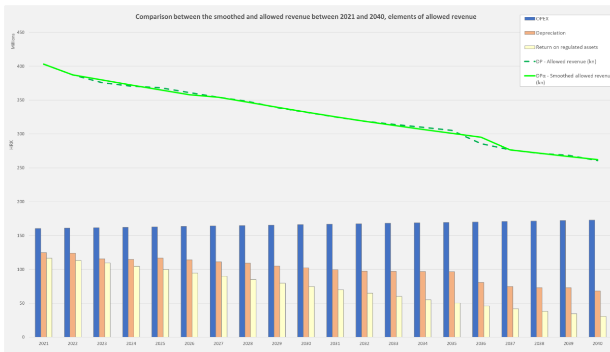
Comparison between the smoothed and allowed revenue between 2021 and 2040.
