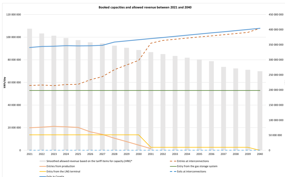
Booked capacities and allowed revenue between 2021 and 2040 forecasted by HERA
