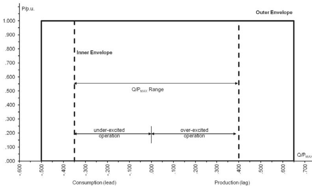
Figure 9 - P-Q/P_{max} -profile of a Power Park Module. The diagram represents boundaries of a P-Q/P_{max} -profile at the Connection Point by the Active Power, expressed by the ratio of its actual value and the Maximum Capacity in per unit, against the ratio of the Reactive Power (Q) and the Maximum Capacity ( P_{max} ). The position, size and shape of the inner envelope are indicative.
