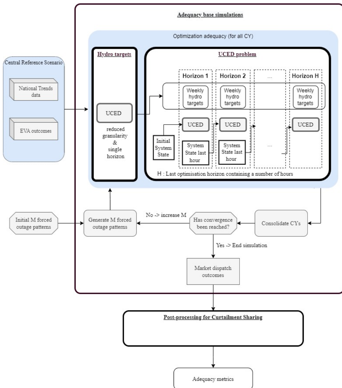
Figure 20: UCED problem
