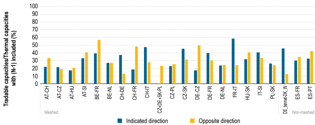
Figure 59: Ratio between available NTC and aggregated thermal capacity of interconnectors – 2015 (%)
